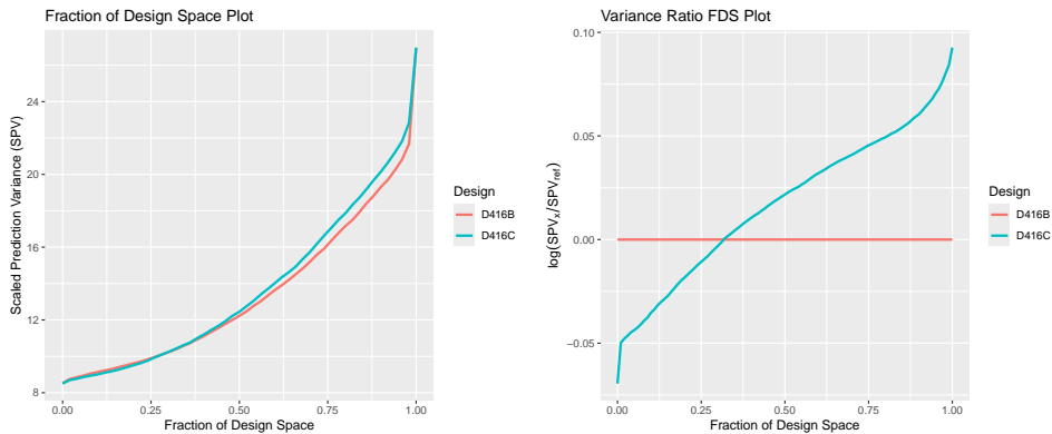
Figure 6: A standard and variance ratio FDS plot for Roquemore’s hybrid designs D416B and D416C for a full quadratic model.
